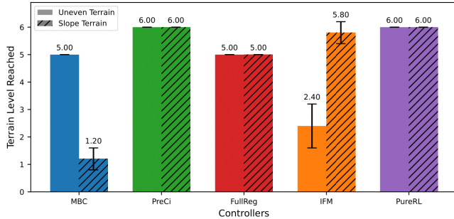
Fig. 5. Terrain level reached by each controller in the MuJoCo robustness test. PreCi successfully traverses all terrains within the time limit. IFM stumbles over its own feet on uneven terrain. FullReg fails to complete the final terrain due to poor tracking performance.
