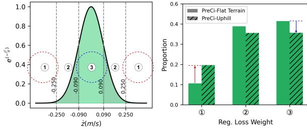
Fig. 7. Left: an adaptive weight distribution against model assumption violation. Right: a histogram of regularization loss weight during PreCi training on both uphill and flat terrain. We observe more unreliable samples with low regularization weight (region 1) and fewer reliable samples with high weight (region 3) in the uphill case, reflecting how PreCi filters out unreliable regularization in violation-prone regions.
