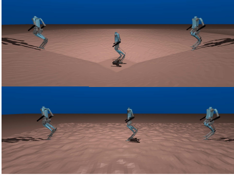
Fig. 4. Sloped (top) and uneven (bottom) terrains used for the robustness tests in MuJoCo.
