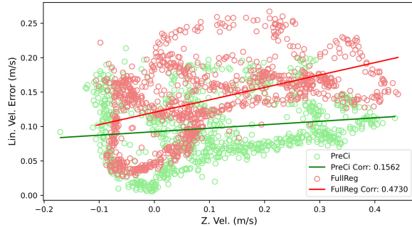
Fig. 8. Relationship between model-assumption violations and linear velocity tracking errors during a 14-degree uphill test. FullReg exhibits higher tracking errors than PreCi when model-assumption violations are more pronounced, while both methods show similar low error distributions when violations are less significant.
