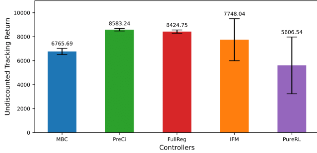
Fig. 6. Mean undiscounted return of tracking rewards in the AR-Sim random velocity tracking test. The command range is wider than that used during training. Policies learned with regularization, PreCi and FullReg, show superior performance compared to those without MBC regularization.
